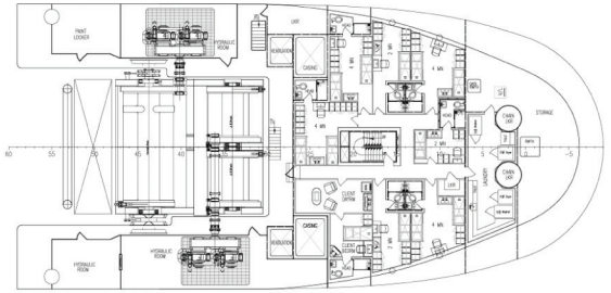
DECK 01
