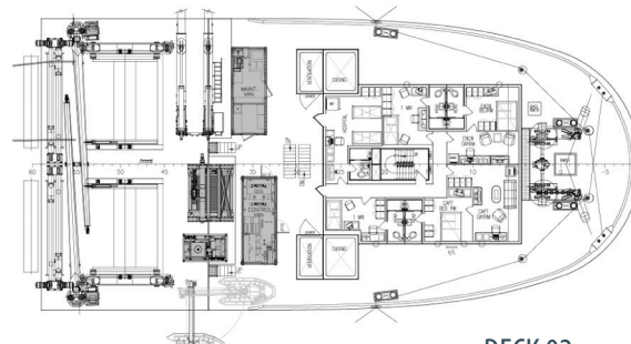
DECK 02
