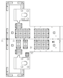
DECK 05
