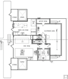
DECK 03
