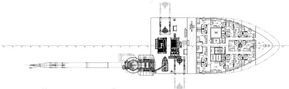
01 DECK PLAN
