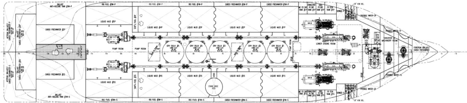
ABOVE TANK-TOP PLAN
